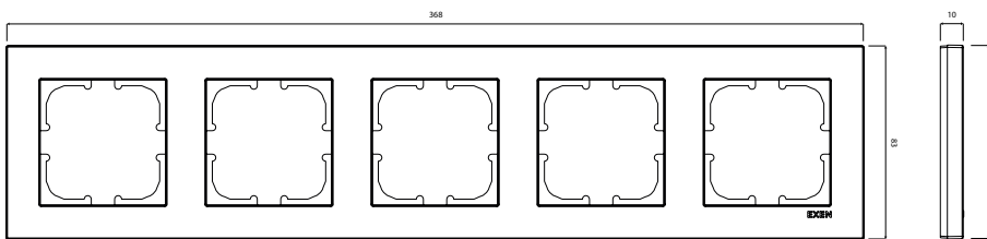
COMFORT Five-Gang Frame
