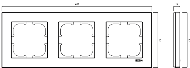
COMFORT Three-Gang Frame
