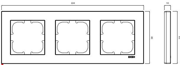
KARELL Three-Gang Frame
