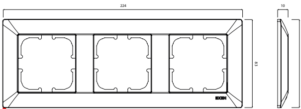
ODAK Three-Gang Frame
