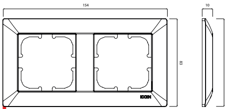
ODAK Two-Gang Frame
