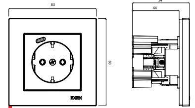
COMFORT Earthed Socket (Schuko) with Type-C
