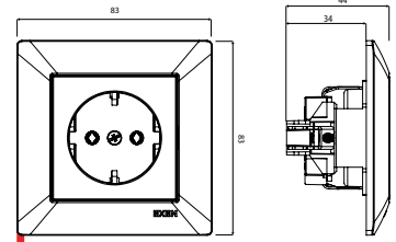
ODAK Earthed Socket (Schuko)
