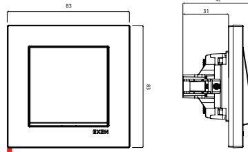
KARELL One Way Switch
