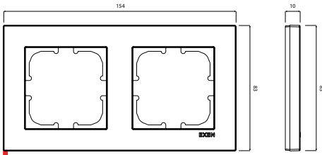
KARELL Two-Gang Frame
