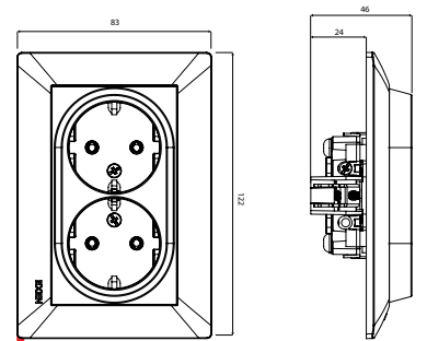
ODAK Two-Gang Earthed Socket
