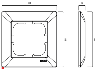
ODAK One-Gang Frame
