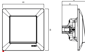
ODAK One Way Switch
