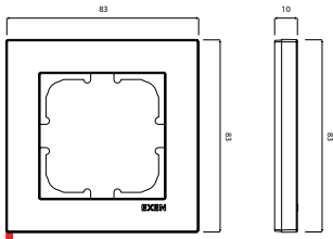
COMFORT One-Gang Frame
