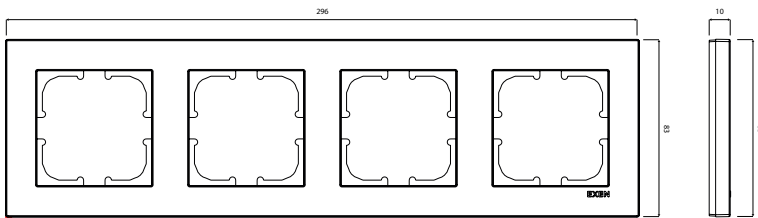
COMFORT Four-Gang Frame
