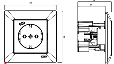
ODAK Earthed Socket (Schuko) with Type-C
