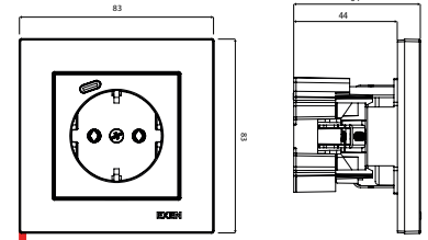
KARELL Earthed Socket (Schuko) with Type-C
