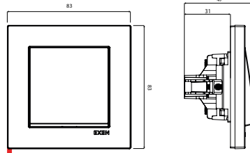
COMFORT One Way Switch
