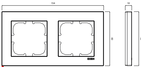
COMFORT Two-Gang Frame
