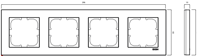
KARELL Four-Gang Frame
