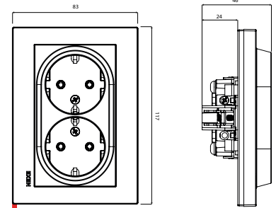
KARELL Two-Gang Earthed Socket
