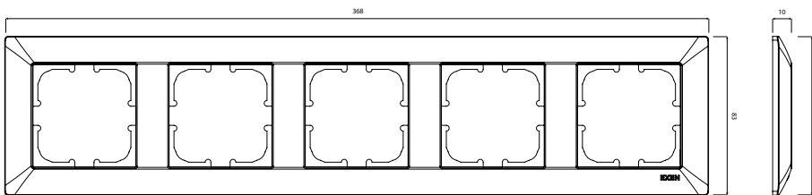
ODAK Five-Gang Frame
