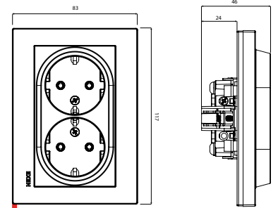
COMFORT Two-Gang Earthed Socket
