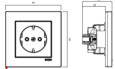
COMFORT Earthed Socket (Schuko)
