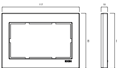
COMFORT Two-Gang Socket Frame
